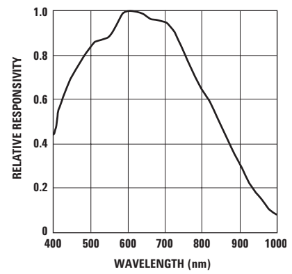
Figure 16. Wavelength Responsivity [1] .
