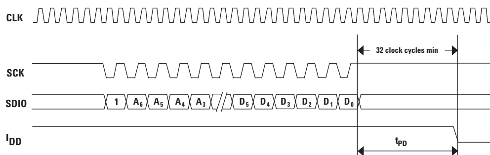
Figure 12. Power-down timing.
