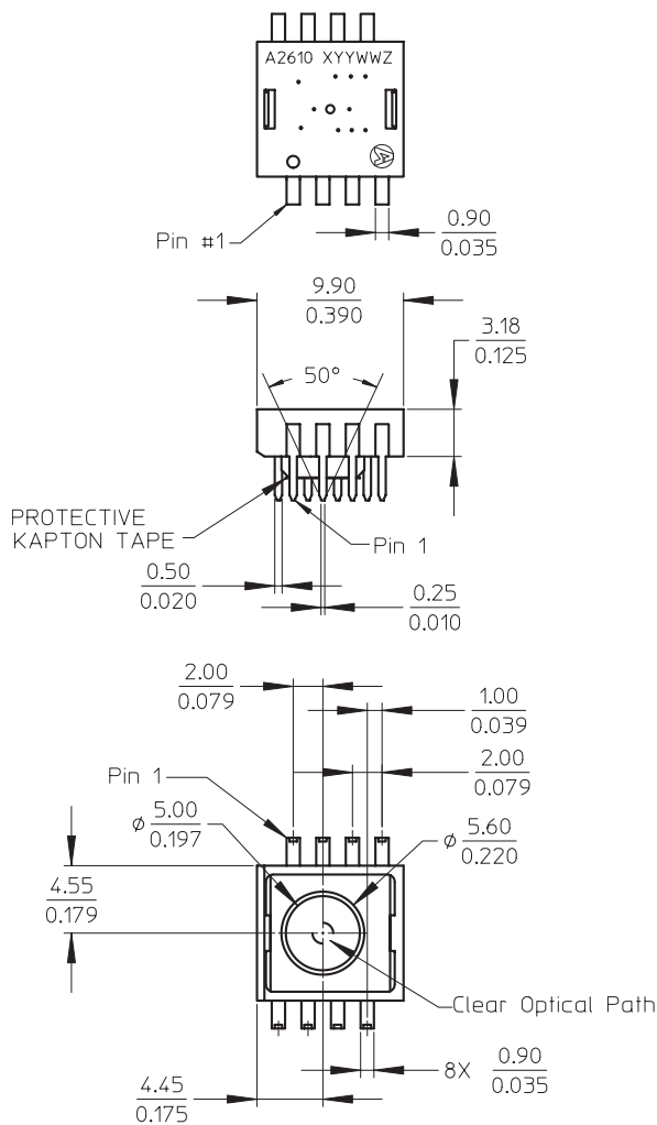
Figure 2. Package outline drawing.
