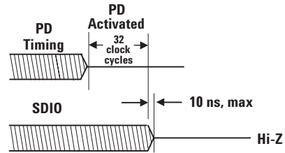
Figure 24. SDIO Hi-z state and timing.
